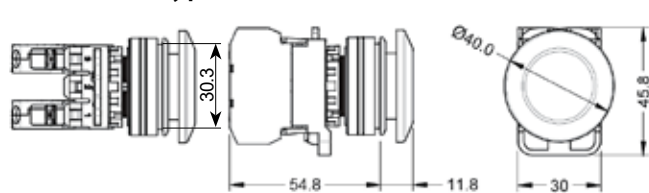
Mushroom type w/flush mountable metal bezels
