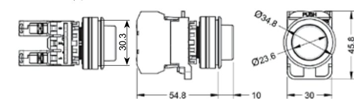
Extended type w/flush mountable metal bezels
