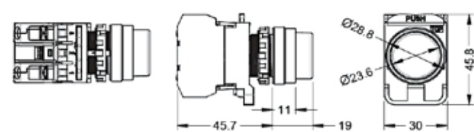
E-Stop switches
