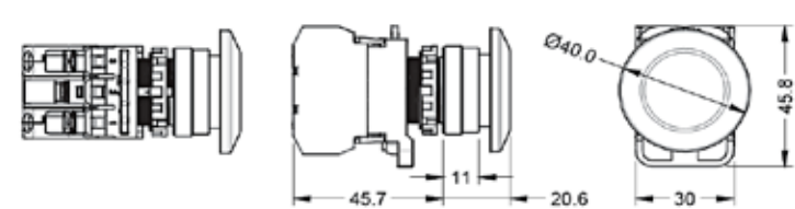
Emergency Switch with Key Reset
