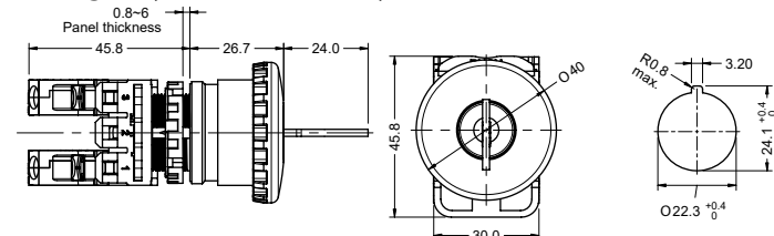
2/3 Position selector switch
