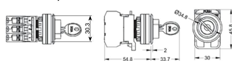
2/3 Position key selector switch w/flush mountable metal bezels
