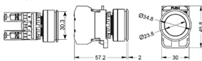
Flush type w/flush mountable metal bezels
