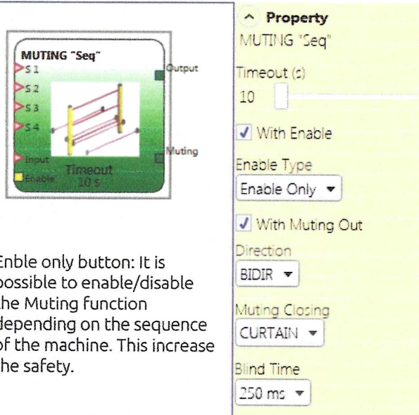
Example of Sequential Muting parameters configuration
