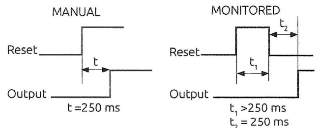
Manual and monitored reset
