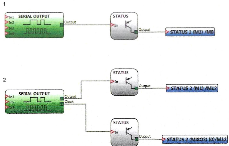
HM1 connections type
