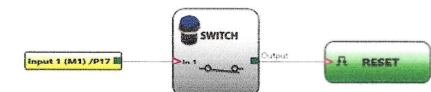
Connection of Reset operator
