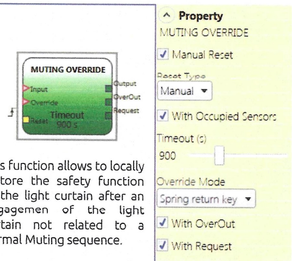
Example of Muting override configuration
