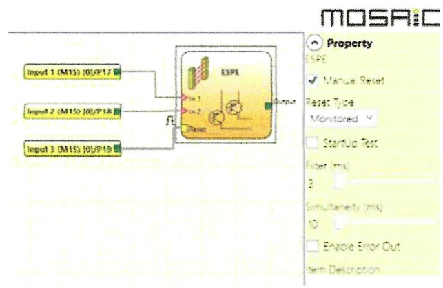
ESPE configuration example
