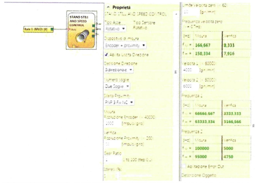
Speed monitoring object configuration example
