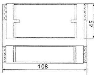
Mosaic M1S COM
