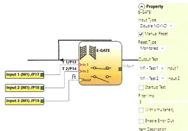
E-gate configuration example
